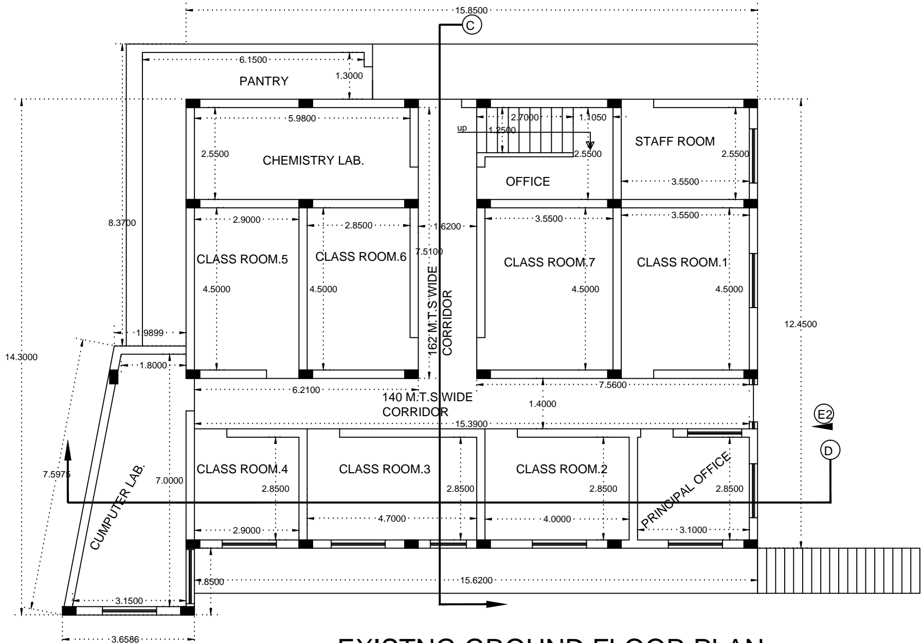
EXISTNG GROUND FLOOR PLAN
