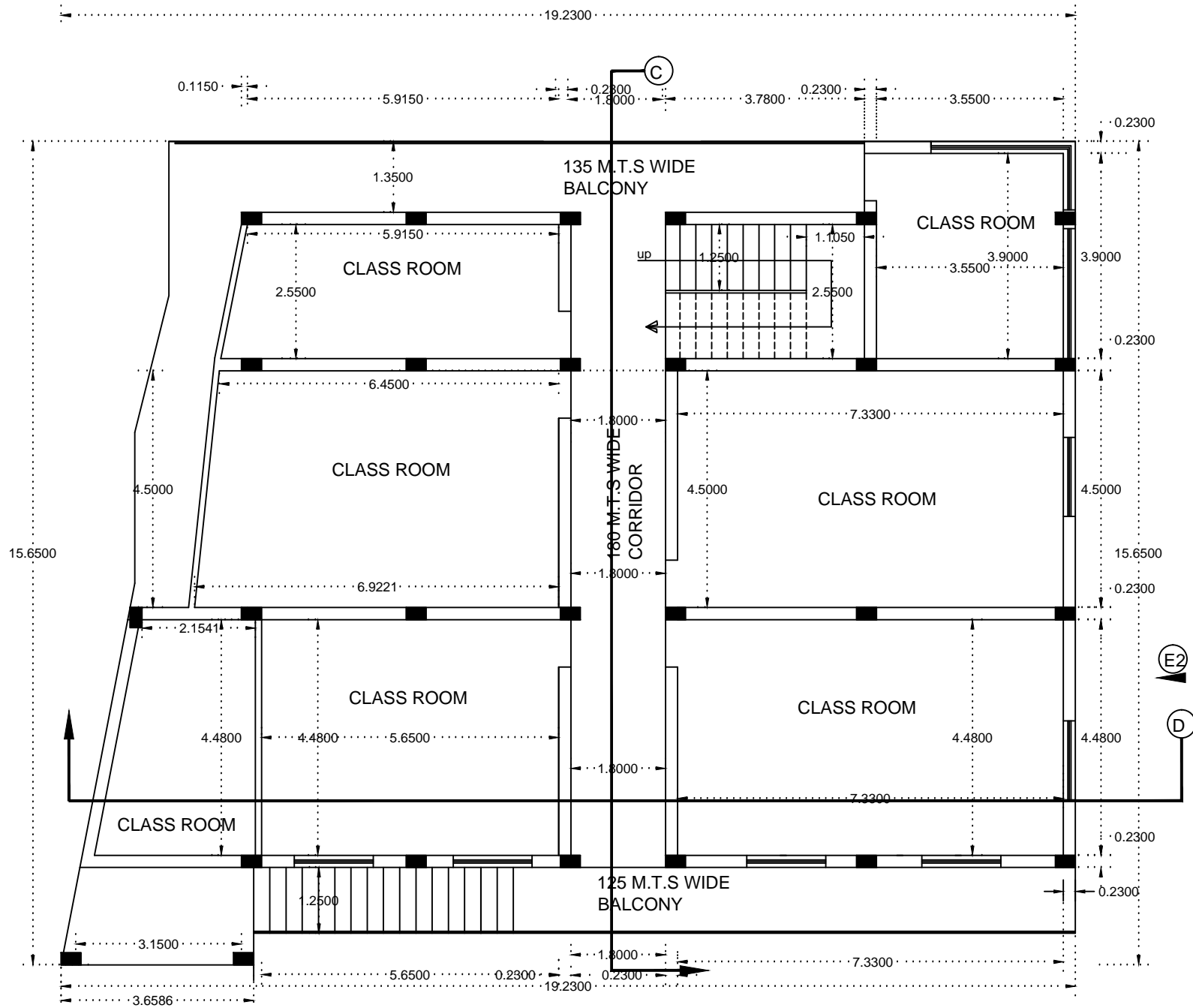
EXISTNG THIRD FLOOR PLAN
