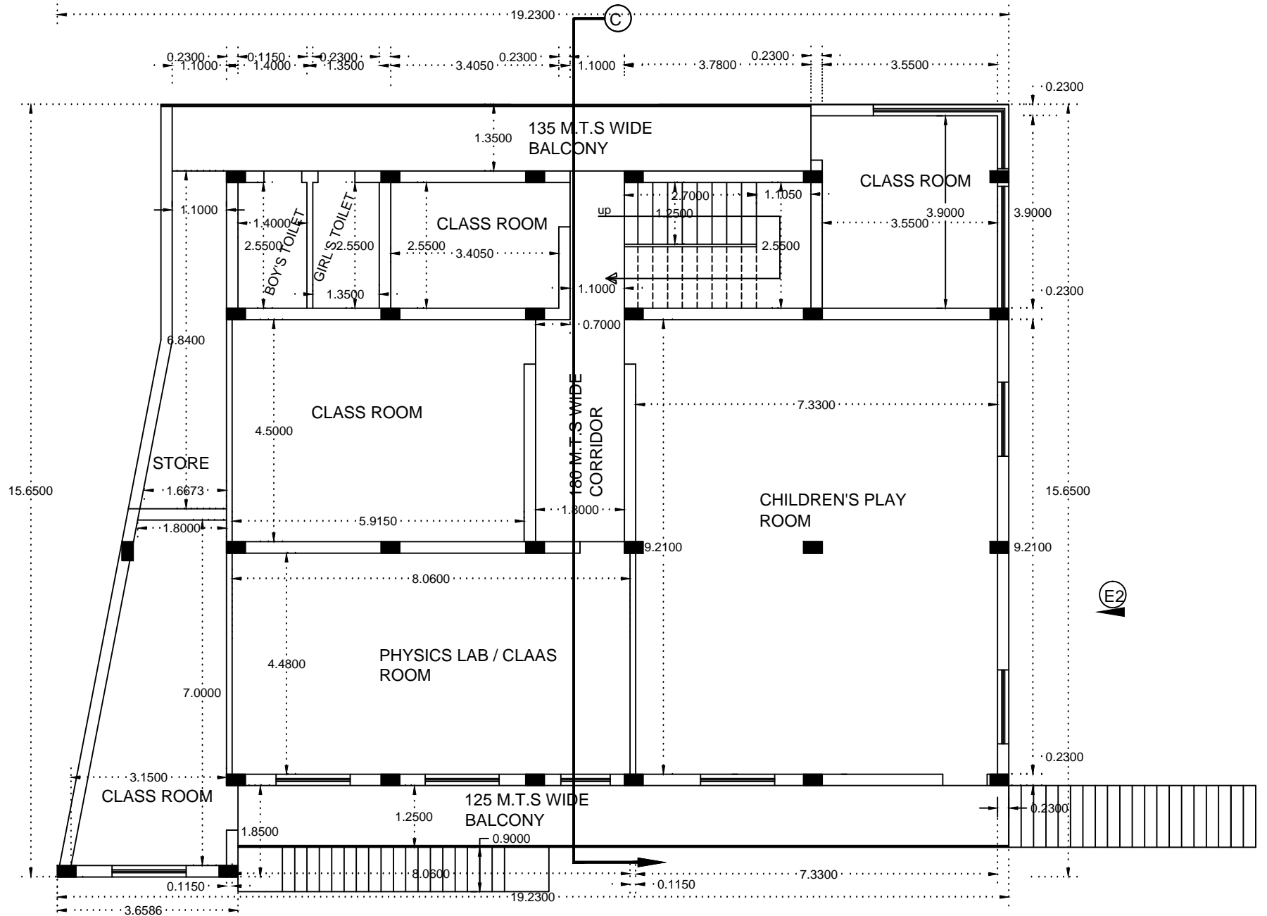
EXISTNG FIRST FLOOR PLAN
