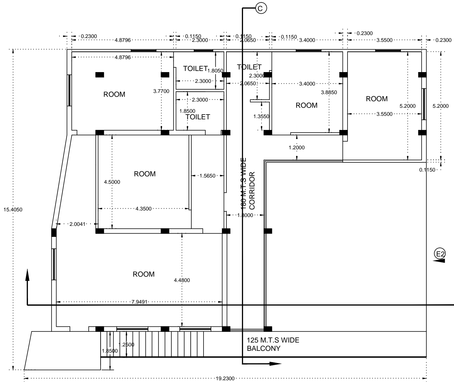
EXISTING FORTH FLOOR PLAN (RESIDENCE)
